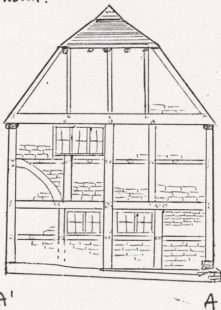
Truss A (outside) facing north.
