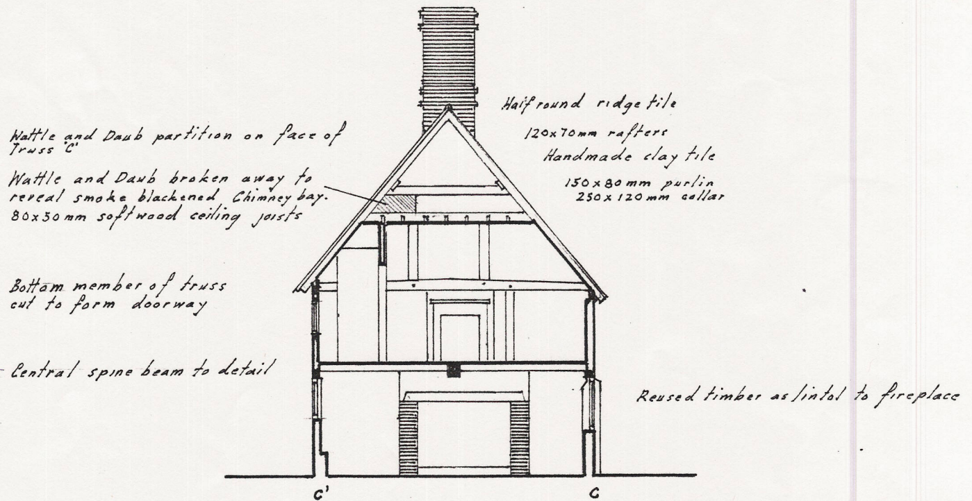
Section at truss 'C'
