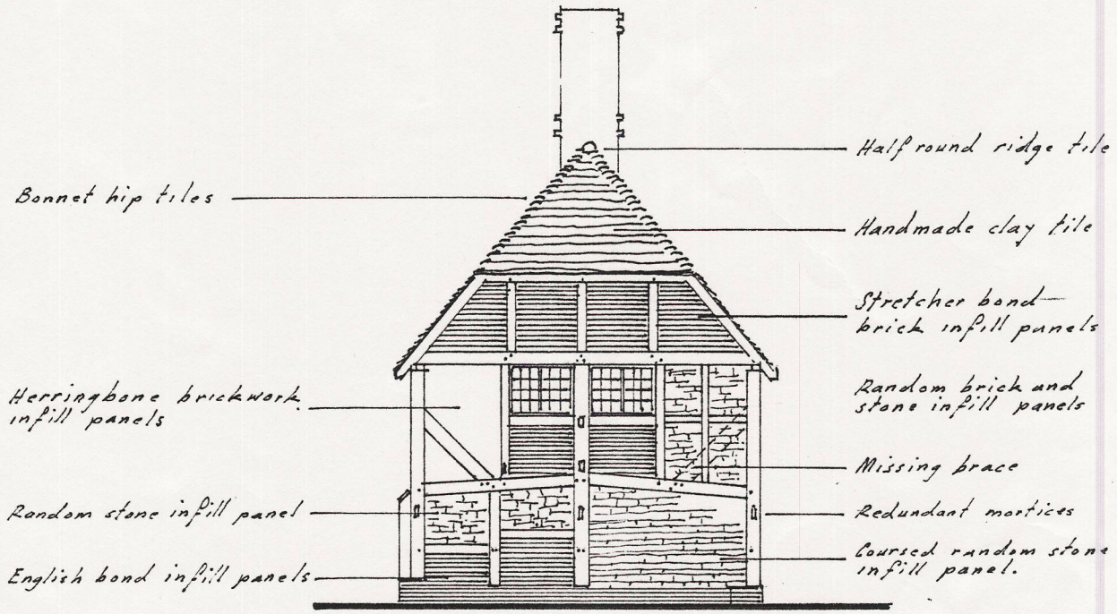
East Elevation
