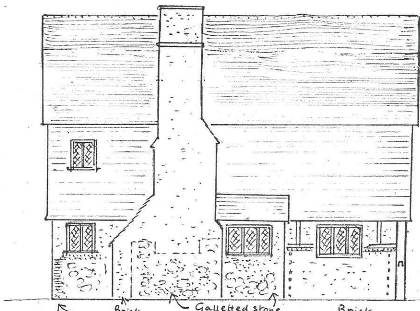
WESTERN ELEVATION
